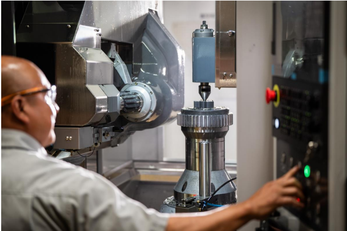
Booth 3609: Helios' Hera 350 CNC Gear Hobbing Machine.
